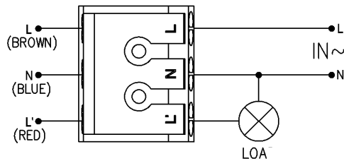
Wandinstallation
