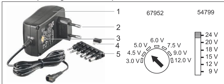
Fig.5: Operating elements and parts
