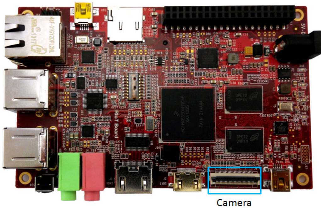
Figure 2-10 Camera Interface
