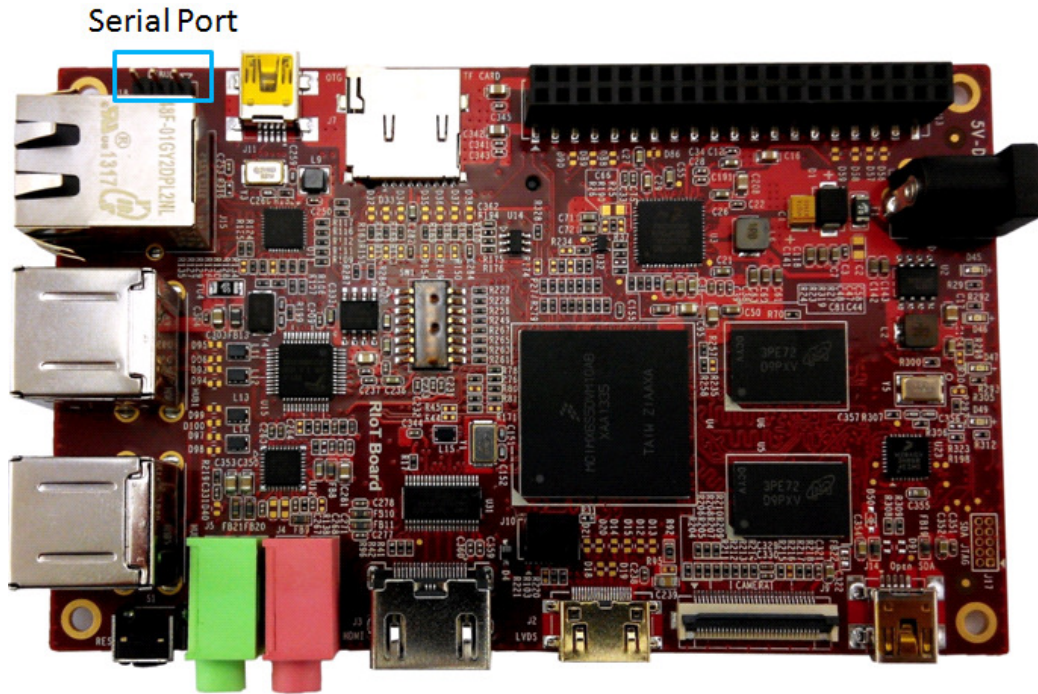
Figure 2-13 Serial Port
