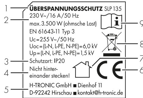
Figure 1 Nameplate
