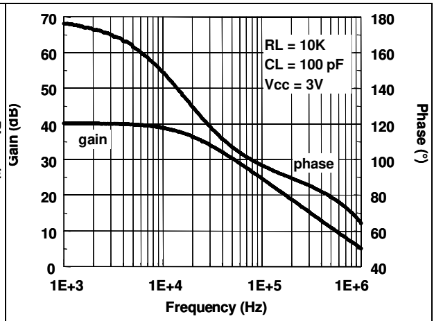
Figure 26. Gain and phase vs. frequency
