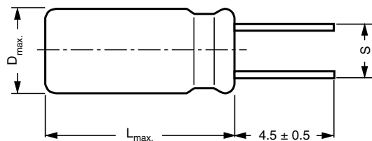
10 ≤ Ø D ≤ 18 Leads shortened and formed EKS 06... (S = 5 / 7.5 mm)
