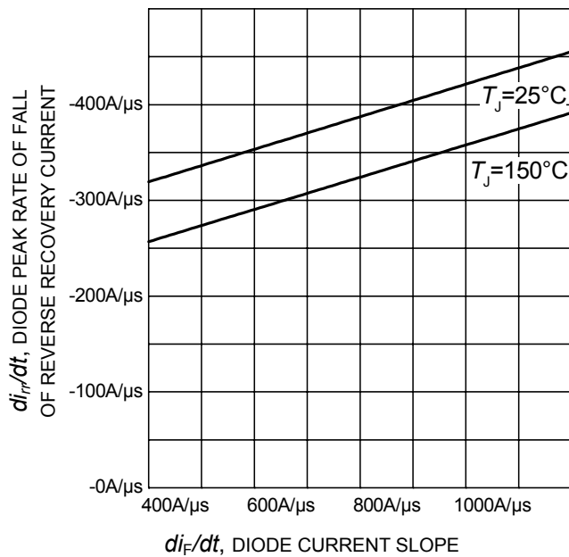
Figure 26. Typical diode peak rate of fall of reverse recovery current as a function of diode current slope ( V_R=600V , I_F=25A , Dynamic test circuit in Figure E)
