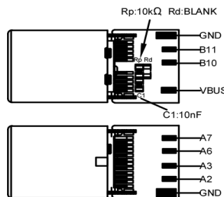
PCB VIEW
