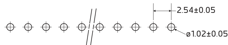
Recommended Board Hole Layout
