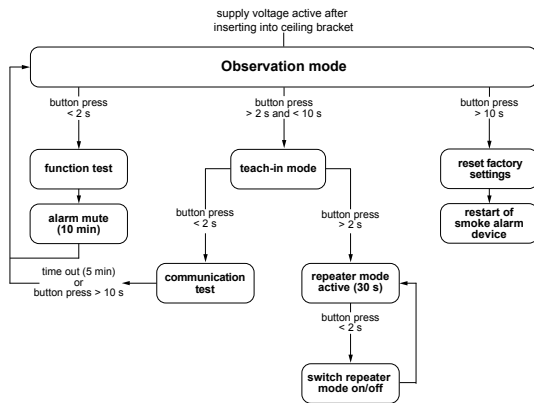
Fig. 13: Operating structure wireless smoke alarm
