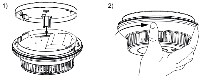
Fig. 11: Latching the wireless smoke alarm device
