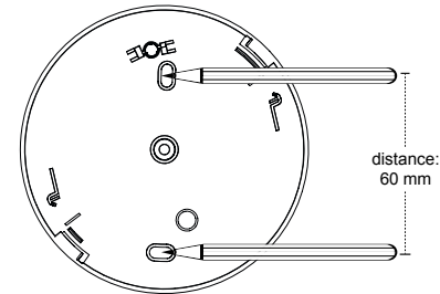
Fig. 12: Marking two bore holes
