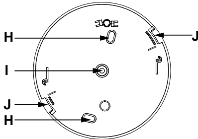
Fig. 3: Ceiling bracket
