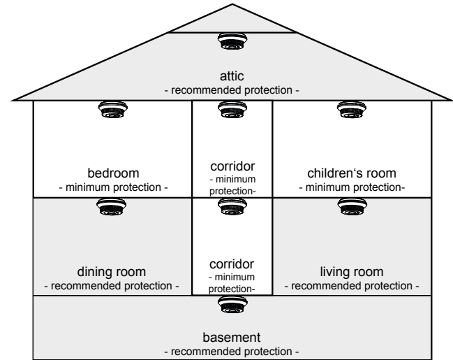
Fig. 8: Mounting wireless smoke alarms - minimum and recommended protection
