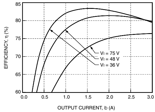
Figure 25. LW015F Typical Efficiency vs. Output Current at T_c = 25\text{ }^\circ\text{C}
