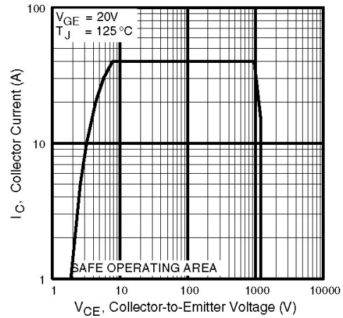
Fig. 12 - Turn-Off SOA
