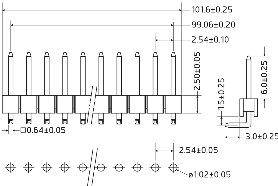
Recommended PCB Board Hole Layout
