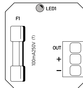
Figure 3 Layout of the electrical connection
