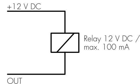
Figure 4 Example of a relay connection
