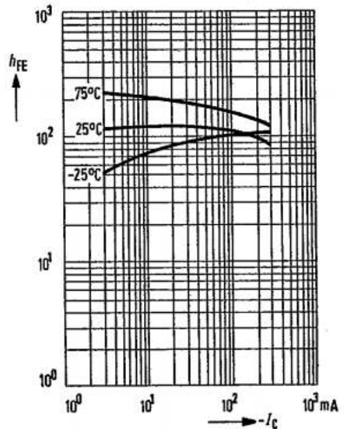
DC current gain h_{FE} = f(I_C) -V_{CE} = 0.5 \text{ V}; T_{amb} = \text{parameter} (common emitter configuration) AC 151, AC 151 r
