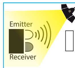
Light interference
