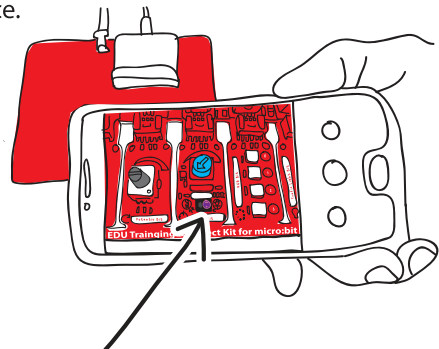
Light interference
