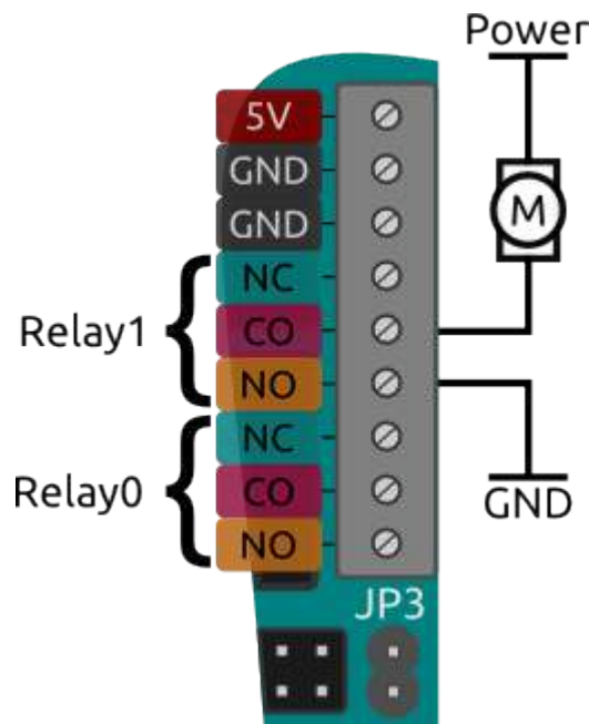
example connection
