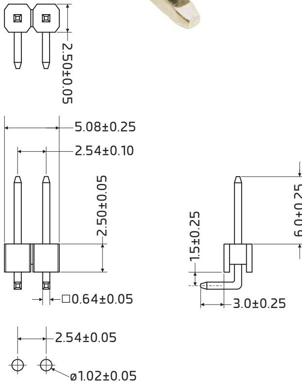
Recommended Board Hole Layout
