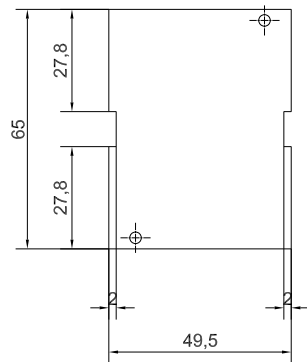
PCB MAX SIZE
