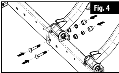
Figure 6: Inserting the retaining screws
