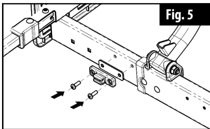
Figure 7: Mounting the retaining clips
