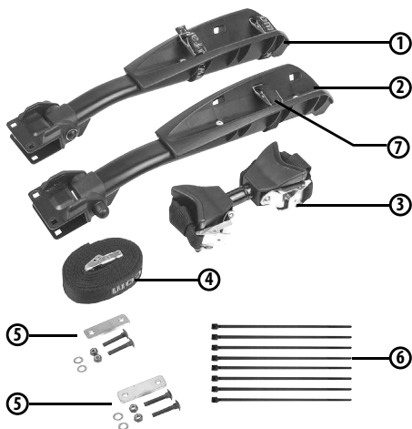
Figure 1 : Fournitures
