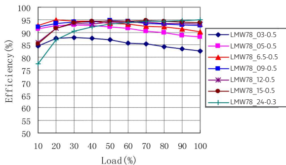
Efficiency VS Load curve (Vin=Vmin)
