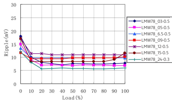
Ripple VS Load curve (Vin=Vmin)
