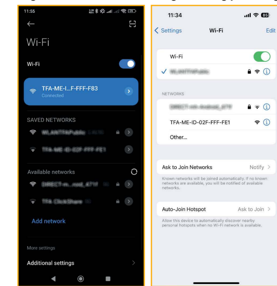
Android iOS
