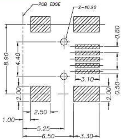
RECOMMENDED PCB LAYOUT (PCB t=0.8)
