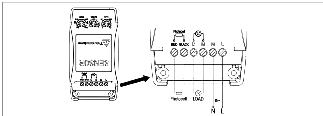
Fig.12: Installation
