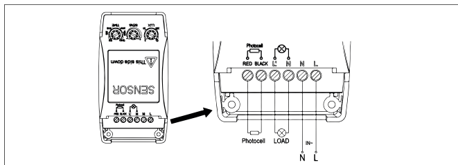
Fig.2: Installation
