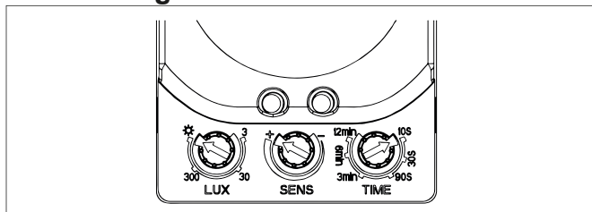
Fig.10: Settings
