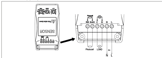
Fig.7: Installation
