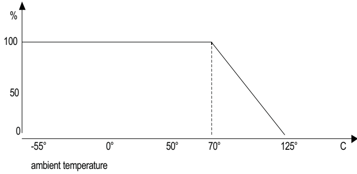
Dissipation as a function of ambient temperature.
