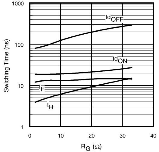
Fig. 14 - Typ. Switching Time vs. R_G
