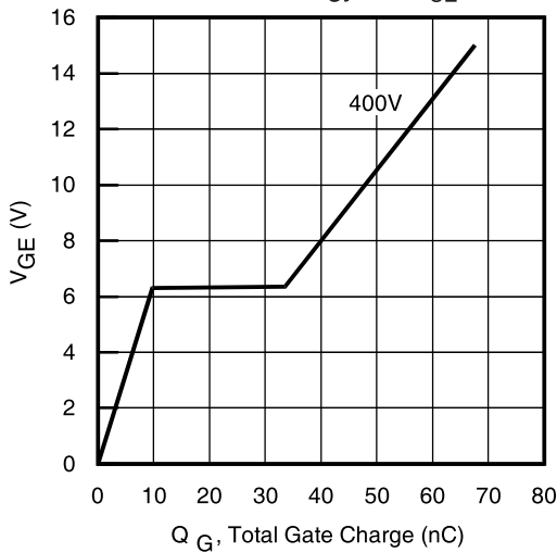
Fig. 17 - Typical Gate Charge vs. V_{GE} I_{CE} = 13A
