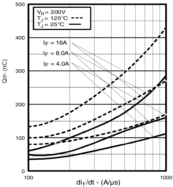
Fig. 21 - Typical Stored Charge vs. di_f/dt
