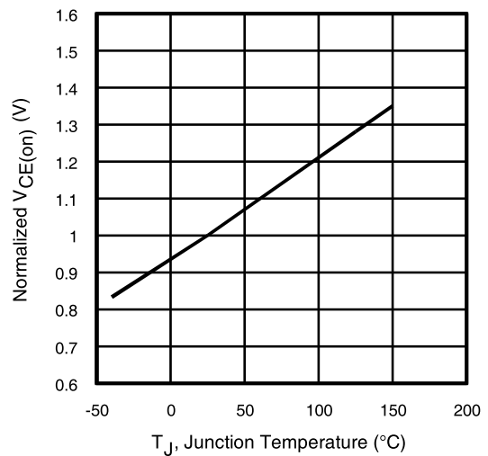
Fig. 18 - Normalized Typical V_{CE(on)} vs. Junction Temperature I_{CE} = 13A , V_{GE} = 15V
