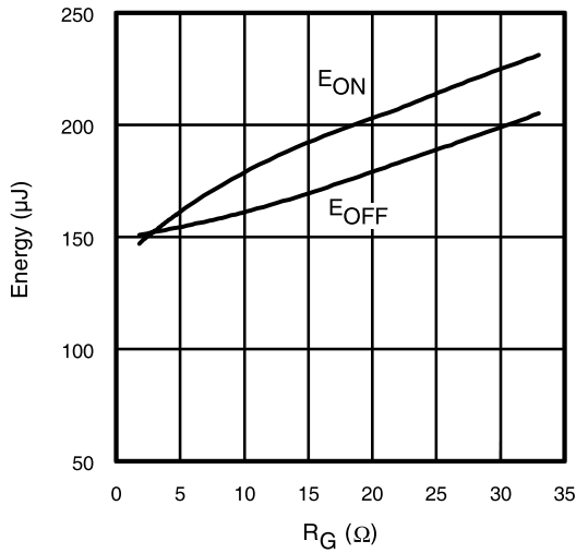
Fig. 13 - Typ. Energy Loss vs. R_G
