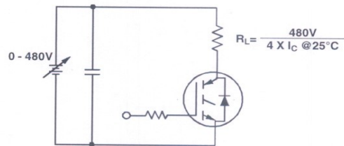
Figure 20. Pulsed Collector Current Test Circuit
