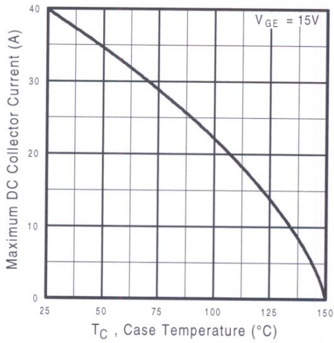
Fig. 4 - Maximum Collector Current vs. Case Temperature
