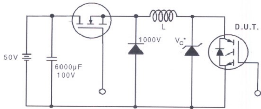
Figure 19. Clamped Inductive Load Test Circuit
