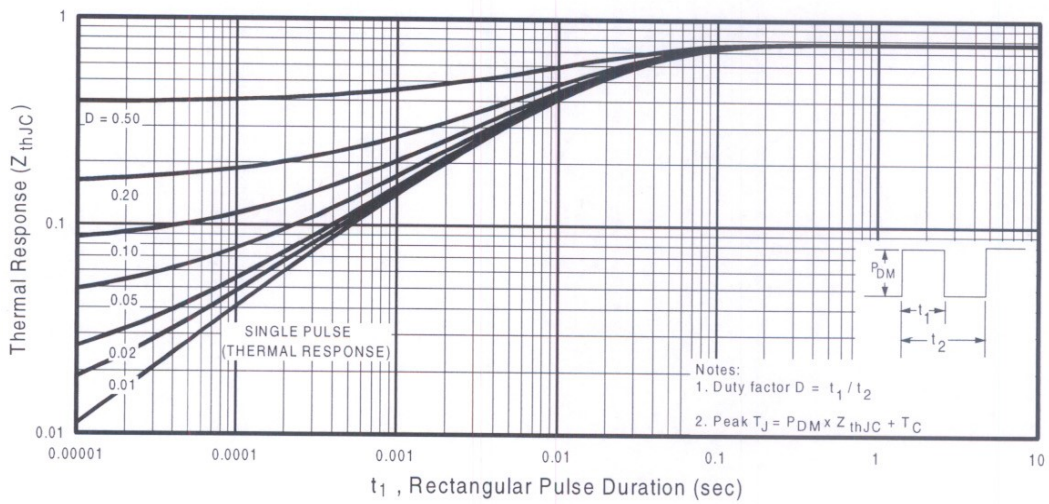
Fig. 6 - Maximum IGBT Effective Transient Thermal Impedance, Junction-to-Case
