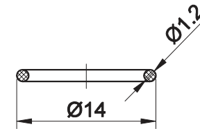
Seal Ring
