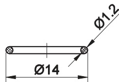
Seal Ring
