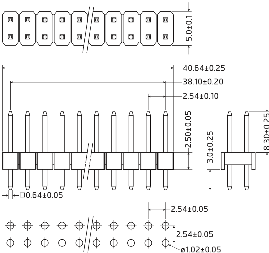
Recommended Board Hole Layout
