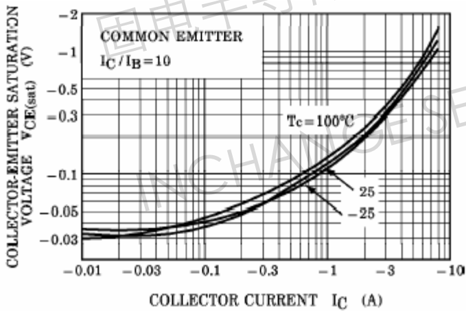
Fig.5 Collector-Emmitter Saturation Voltage
