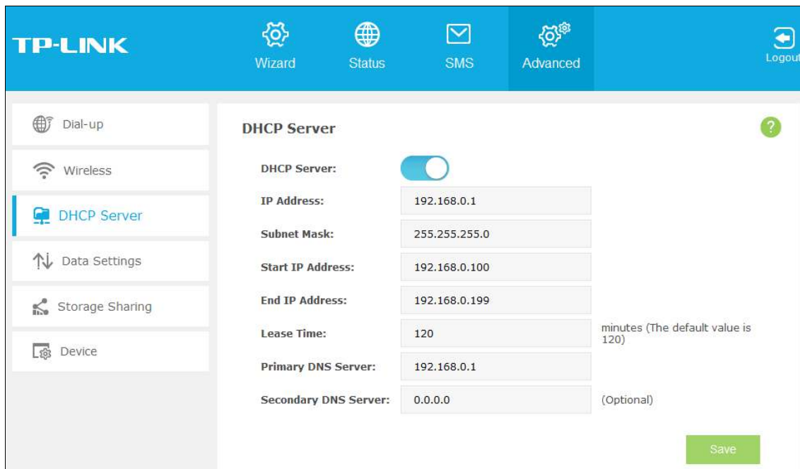
Figure 4-22 DHCP Server
